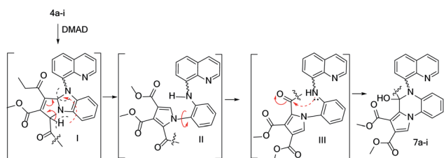
Scheme 2 Reaction mechanism for obtaining dihydro-pyrrolo-quinoline quinoline compounds 7a-i .
