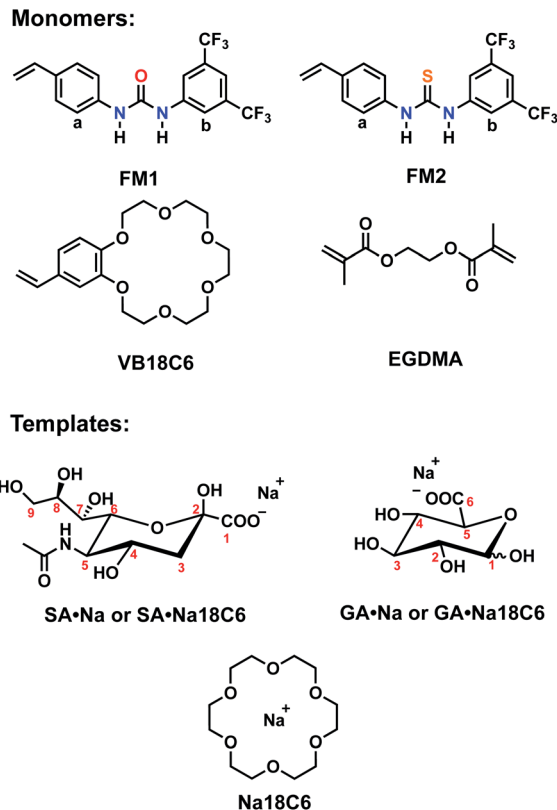
Fig. 2 Structures of functional monomers and templates with corresponding counterions.
