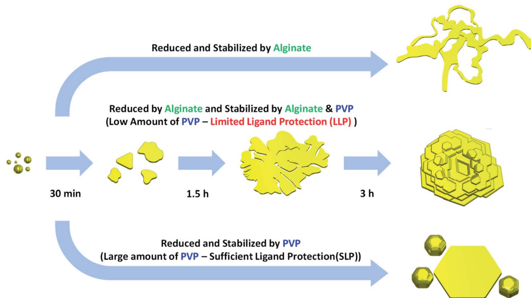
Fig. 5 Schematic of the shape changes of Au nanocrystals depending on the amount of PVP, which was used as a capping ligand in the present study. The rose-shaped Au nanostructures can be formed in the special reaction region corresponding to limited ligand protection (LLP).
