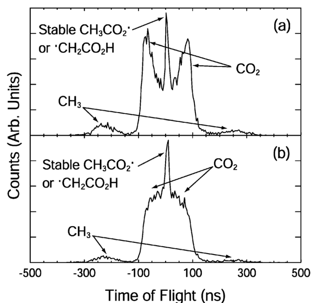
Fig. 2 The fragment TOF spectra for \text{CH}_3\text{CO}_2^- at 3.5 eV with the electric vector of the laser (a) parallel and (b) perpendicular to the direction of ion beam. 10 Reprinted with permission from Journal of Physical Chemistry A , 2004, 108, 9962. Copyright 2004 American Chemical Society.
