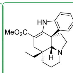
136 : (+)-Vincadifformine
