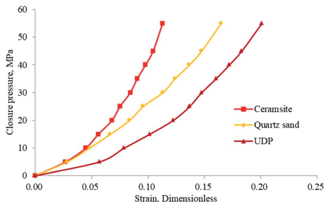
Fig. 15 Strain of different proppant at different closure pressures.
