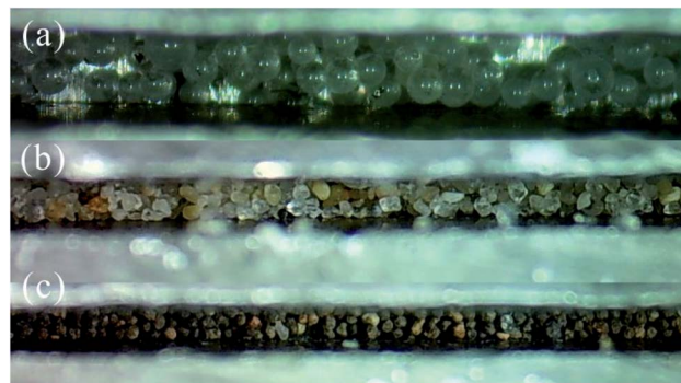
Fig. 12 The morphology images of UDP, quartz sand and ceramics.
