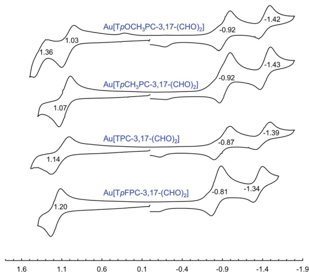
Fig. 10 Cyclic voltammograms (V vs. SCE) for Au[TPXPC-3,17-(CHO) 2 ] derivatives in dichloromethane containing 0.1 M TBAP.
