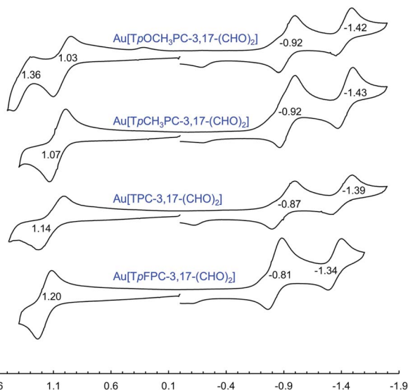
Fig. 10 Cyclic voltammograms (V vs. SCE) for Au[TPXPC-3,17-(CHO) 2 ] derivatives in dichloromethane containing 0.1 M TBAP.
