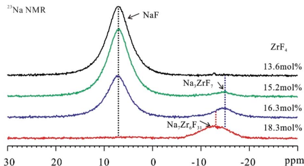
Fig. 3 ^{23}\text{Na} NMR spectra of FLiNaK–ZrF 4 ( 13.6 \leq X_{\text{ZrF}_4} \leq 18.3 \text{ mol\%} ) eutectic solidification salts at ambient temperature. MAS spin rate in the mentioned experiments was set to 15 kHz.
