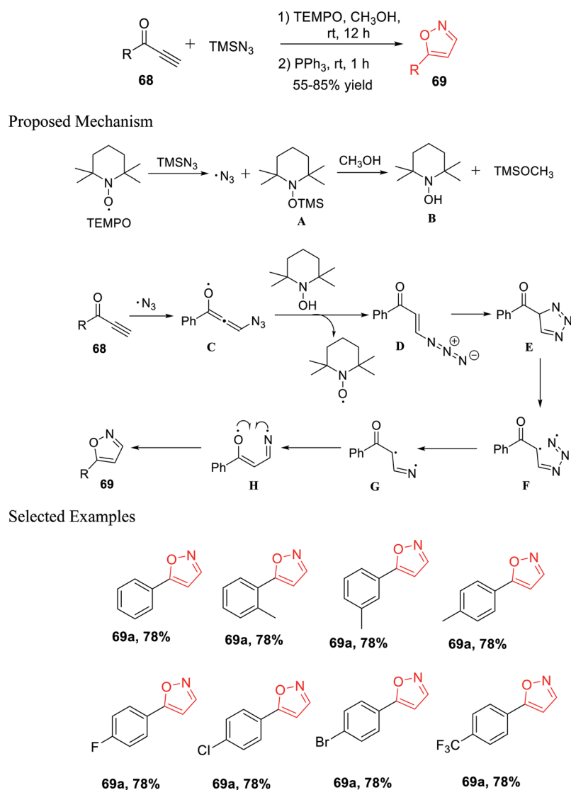
Scheme 16 Synthesis of 5-substituted isoxazole using the TEMPO catalyst.
