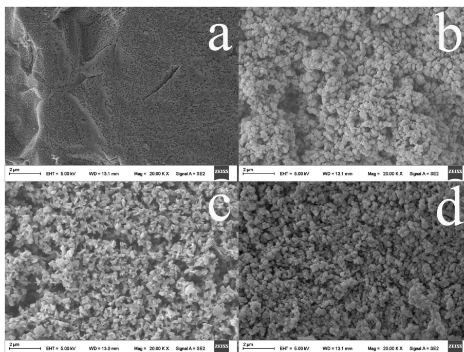
Fig. 1 SEM images of the commercial Ti wire (a), the TiO 2 NPs/Ti fiber (b), the annealed TiO 2 NPs/Ti fiber (c), and the PPy@TiO 2 NPs/Ti coated fiber (d).
