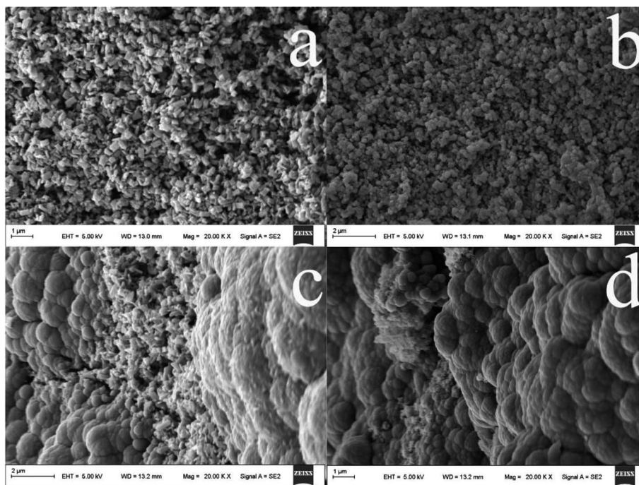
Fig. 3 SEM images of PPy@TiO 2 NPs at electropolymerization voltages of 2 V (a), 4 V (b), 6 V (c) and 8 V (d).
