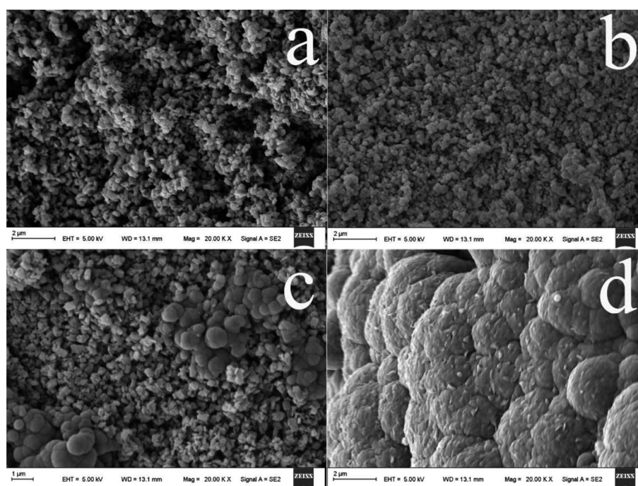
Fig. 2 SEM images of the PPy@TiO 2 NPs coating at a pyrrole concentration of 0.02 mol L -1 (a), 0.05 mol L -1 (b), 0.08 mol L -1 (c) and 0.1 mol L -1 (d).
