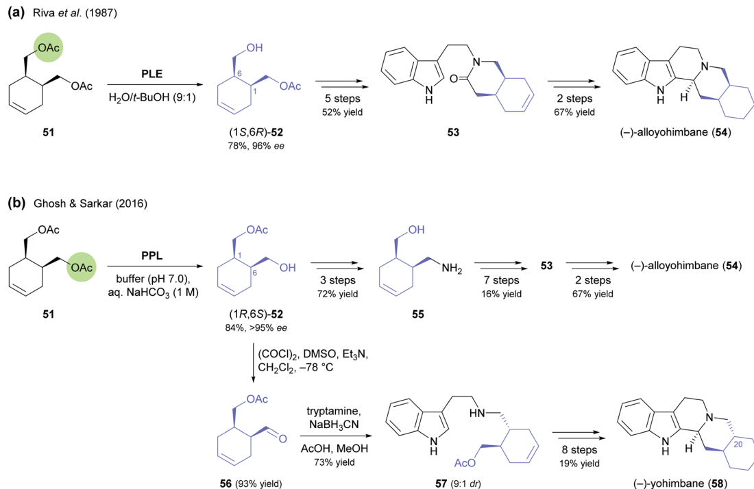
Scheme 8 Preparation of building block 52 by hydrolase-catalysed desymmetrisation and its use in the synthesis of yohimbe alkaloids: (a) synthesis of (-)-alloyohimbane (54) from (1 S ,6 R )-52, (b) synthesis of (-)-alloyohimbane (54) and (-)-yohimbane (58) from (1 R ,6 S )-52.
