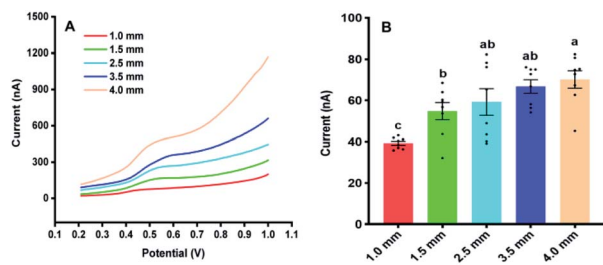
Fig. 4 The Influences of the sampling area on the electrochemical responses of IAA in Arabidopsis thaliana leaves. (A) The DPV curves of IAA in plant samples with different areas. (B) The contents of IAA in the plant samples with the different areas. All experiments were repeated eight times. Data are shown as means \pm SEM. Bars with different letters indicate significant differences at p < 0.05 by two-way ANOVA with Tukey's multiple comparison test.
