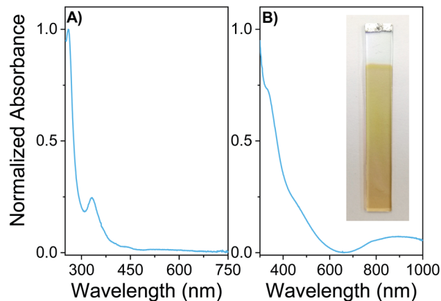
Fig. 3 (A) Electronic absorption spectrum of EDOT-C 60 monomer in DCM at room temperature. (B) Absorption spectrum of PEDOT-C 60 film on ITO. The inset shows a photo of the polymer PEDOT-C 60 deposited on ITO.
