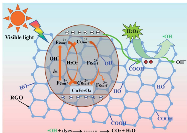
Fig. 8 Schematic illustration of an active heterogeneous photo-Fenton mechanism based on CoFe 2 O 4 -RGO hybrids.
