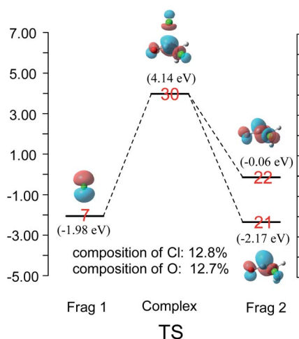
Fig. 5 Schematic molecular orbital interaction diagram showing the transition state of the reaction of \text{Cl}^- and acyl chloride (isosurface = 0.05 a.u.). Frag 1 and Frag 2 are fragments of \text{Cl}^- and acyl chloride, respectively.
