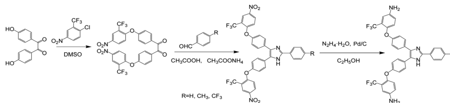
Scheme 1 Synthesis routes of the intermediate BNTFPED, PBNI, MPBNI, TFPBNI and the diamine PBAl, MPBAl, TFPBAl.
