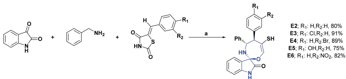
Scheme 50 Structures, reagents and conditions for the synthesis of spiro heterocycles [4.6.0] E2 – E6 . (a) \text{Et}_3\text{N} , THF, reflux, 20 min.
