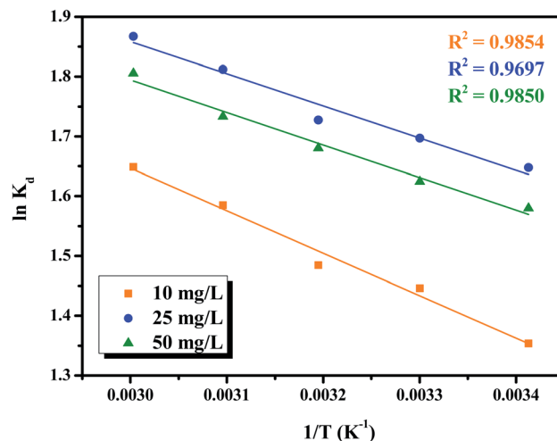
Fig. 5 Van't Hoff plot for the adsorptive removal of Cr(vi) ions (concentration = 10.0 , 25.0 , and 50.0 \text{ mg L}^{-1} ) on the \text{NFe}_3\text{O}_4\text{Starch-Glu-NFe}_3\text{O}_4\text{ED} nanocomposite.
