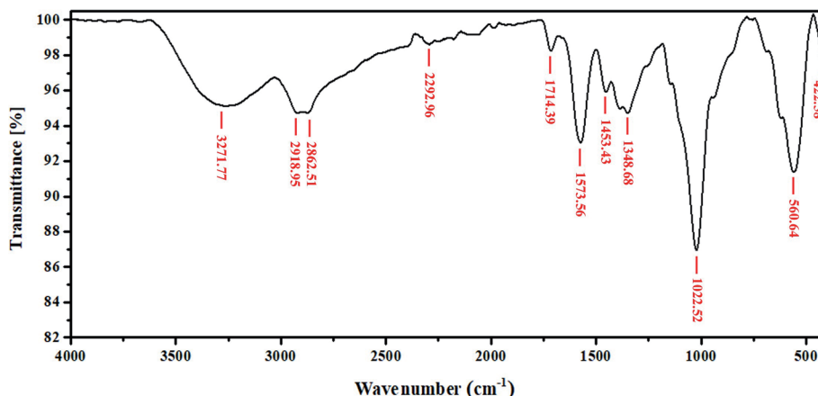
Fig. 1 FT-IR spectrum of the NFe 3 O 4 Starch-Glu-NFe 3 O 4 ED nanocomposite.
