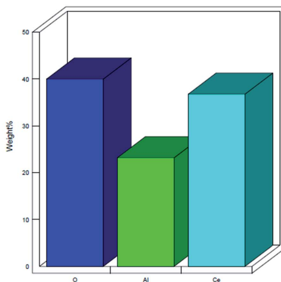
Element Weight% Atomic% O K 40.02 69.03 Al K 23.20 23.72 Ce L 36.78 7.24 Totals 100.00
