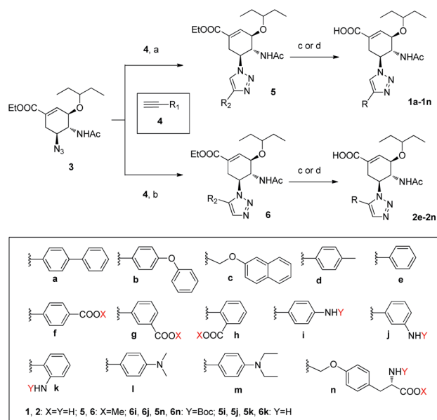
Scheme 1 Synthesis of target compounds. Reagents and conditions: (a) sodium ascorbate, aq CuSO 4 , THF/H 2 O (3 : 1), 45 °C, 6–12 h, 68–98%; (b) Cp* 2 RuCl(PPh 3 ) 2 , THF, 60 °C, 12–24 h, 29–89%; (c) aq NaOH, MeOH, rt, 6–12 h, 55–81%; (d) (i) aq NaOH, MeOH, rt, 6–12 h; (ii) TFA/DCM (1 : 1), rt, 3–4 h, 72–79%.
