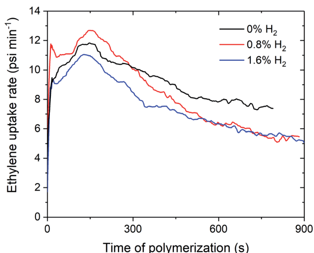
Fig. 2 Slurry-phase polymerisation ethylene uptake rate as a function of time of polymerisation using sMAO supported Me 2 SB( t BuN 2 I*)TiCl 2 ( 1 s MAO ) with 0 (black), 0.8 (red), and 1.6% H 2 (blue). Polymerisation conditions: 8.3 bar ethylene, 0.20 mg pre-catalyst ([Al] sMAO /[Ti] 0 = 200), 5.0 mL heptane, 10 μmol TiBA, and 80 °C. Reactions quenched at 8.3 bar ethylene uptake or after 60 minutes.
