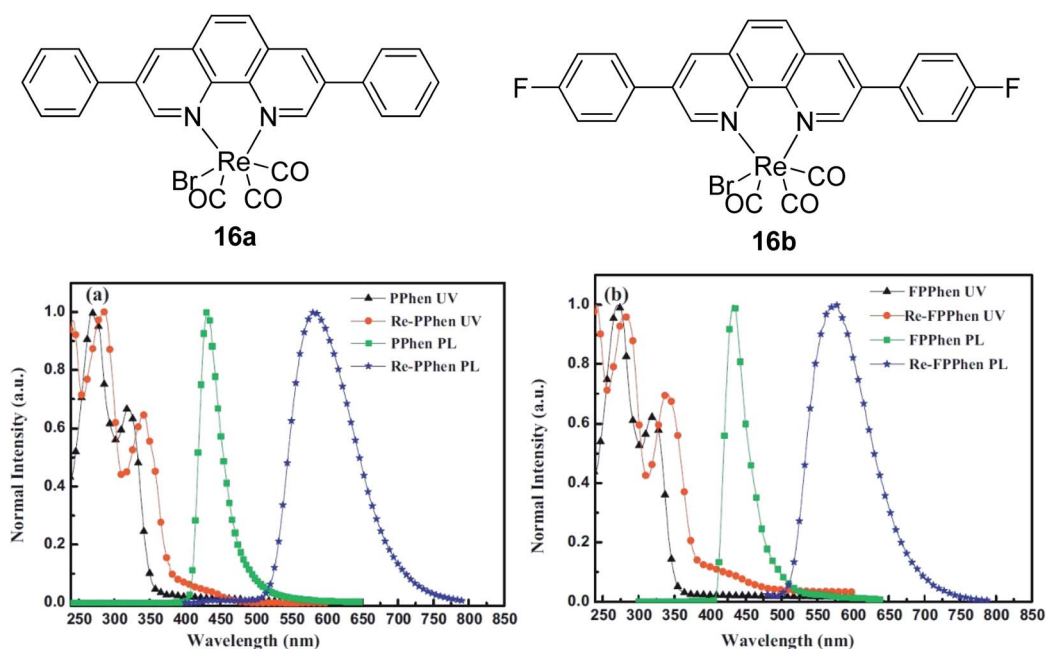
Fig. 23 Molecular structure of rhenium(I) complexes (16a and 16b), and their absorption and emission spectra in dichloromethane. (PPhen = 3,8-diphenyl-1,10-phenanthroline; Re-PPhen = 16a; FPhen = 3,8-bis(4-fluorophenyl)-1,10-phenanthroline; Re-FPPhen = 16b). The figure was adapted from ref. 134 with copyright permission from Elsevier.
