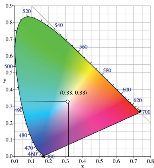
Fig. 1 The chromaticity coordinates ( x , y ) of pure white light, as given by the Commission Internationale d'Eclairage, is (0.33, 0.33). The figure was adapted from ref. 25 with accreditation given to Creative Commons Attribution 4.0 International Public License.
