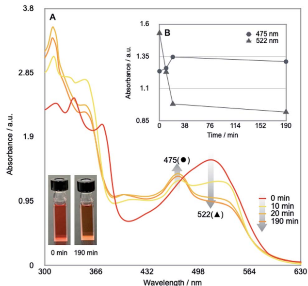
Fig. 2 (A) Time-dependent UV-Vis absorption spectra of Me-Cbl in DMF ( 10^{-4} mol L ^{-1} ) under the blue-light irradiation under argon atmosphere. (B) Variation over time of absorbances at 475 and 522 nm.
