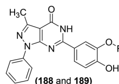
Fig. 61 Chemical structures of selected pyrazolopyrimidines (188 and 189).
