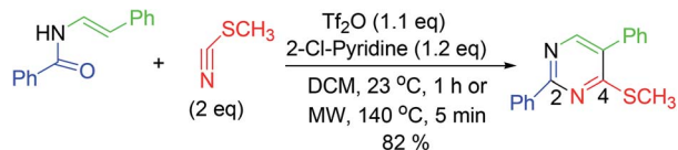
Scheme 9 Synthesis of C 4 -heteroatom substituted pyrimidines.
