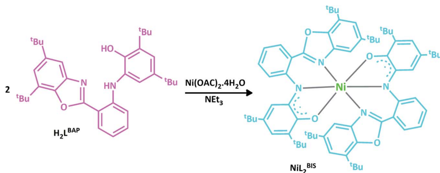
Scheme 2 The structure of H_2L^{BAP} and the associated NiL_2^{BIS} complex.
