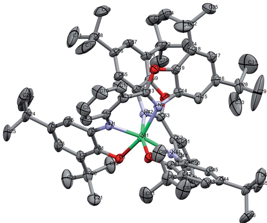
Fig. 1 Molecular structure of \text{Ni}^{\text{II}}\text{L}_2^{\text{BIS}} , H atoms have been omitted for clarity. Thermal ellipsoids are set at 30% probability.
