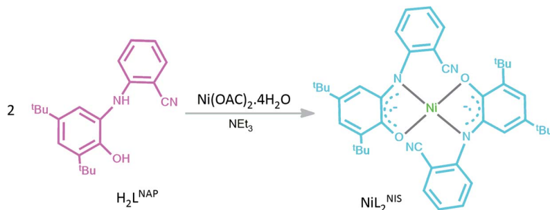
Scheme 3 The structure of H_2L^{NAP} and the associated NiL_2^{NIS} complex. 1
