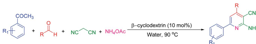
Scheme 1 One-pot four-component synthesis of 2-amino-4,6-diphenylnicotinonitriles.
