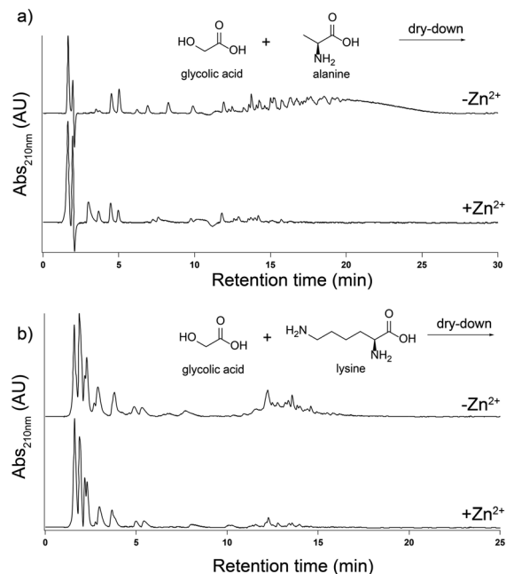
Fig. 2 Zinc does not increase extent of polymerization or length of oligomers of Ala- or Lys-containing depsipeptides in dry-down reactions. Alanine (a) or lysine (b) were dried with glc at a 1 : 1 molar ratio, for one week at 85 °C under unbuffered conditions, in the presence or absence of Zn^{2+} , at a 1 : 1 molar ratio of amino acid to Zn^{2+} . The addition of Zn^{2+} hindered depsipeptide formation for both amino acids tested, as opposed to the reverse trend observed with His.
