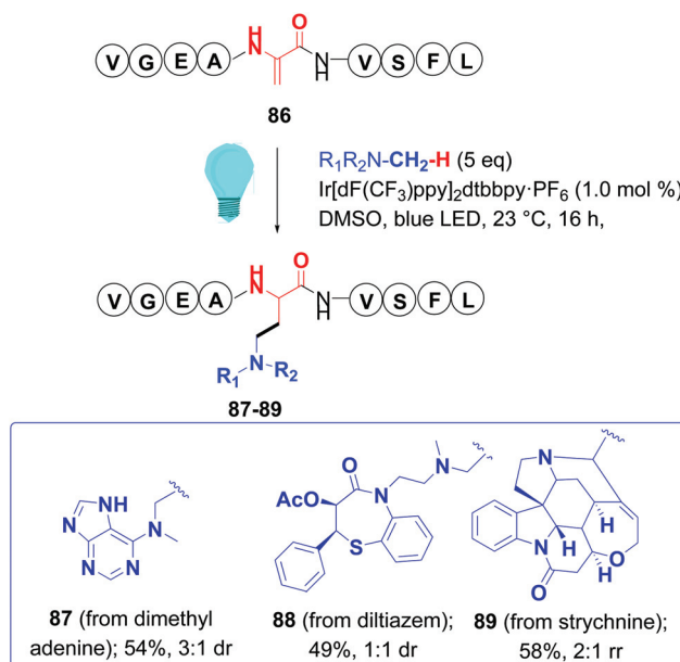
Scheme 22 Peptide functionalization with C-radicals by Jui et al. 79
