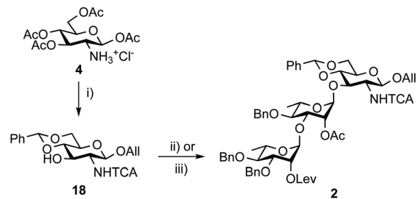
Scheme 4 Synthesis of trisaccharide 2 from tetraacetate 4 . (i) a. Cl 3 CC(O)Cl, pyridine, DCM; b. AlOH, TMSOTf, DCM; c. NaOMe, MeOH; d. PhCH(OMe) 2 , CSA, MeCN, 88%. 50 (ii) 17 , TMSOTf, 4 Å MS, DCM, 0 °C to rt, 86% (45 g scale). (iii) Crude 17 from 15 , TMSOTf, 4 Å MS, DCM, 0 °C to rt, 97% (11 g scale). TCA: trichloroacetyl.
