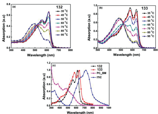
Fig. 26 Temperature-dependent absorption spectra of (a) 132 and (b) 133 in chlorobenzene solution, and (c) absorption spectra of 132 , 133 , PC 71 BM and ITIC in film. Reproduced with permission of Elsevier. 77
