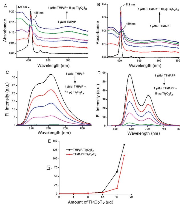
Fig. 1 Changes in the UV-visible absorption and fluorescence emission of 1 \mu\text{M} of TMPyP (A and C) and 1 \mu\text{M} of TTMAPP (B and D), upon titration with 0.2 \text{ mg mL}^{-1} of \text{Ti}_3\text{C}_2\text{T}_x in water, respectively. (E) The graph shows the extent of emission quenching with respect to the amount of the \text{Ti}_3\text{C}_2\text{T}_x ( I_0 and I are the intensity at fluorescence maxima of porphyrins before and after adding \text{Ti}_3\text{C}_2\text{T}_x , respectively).
