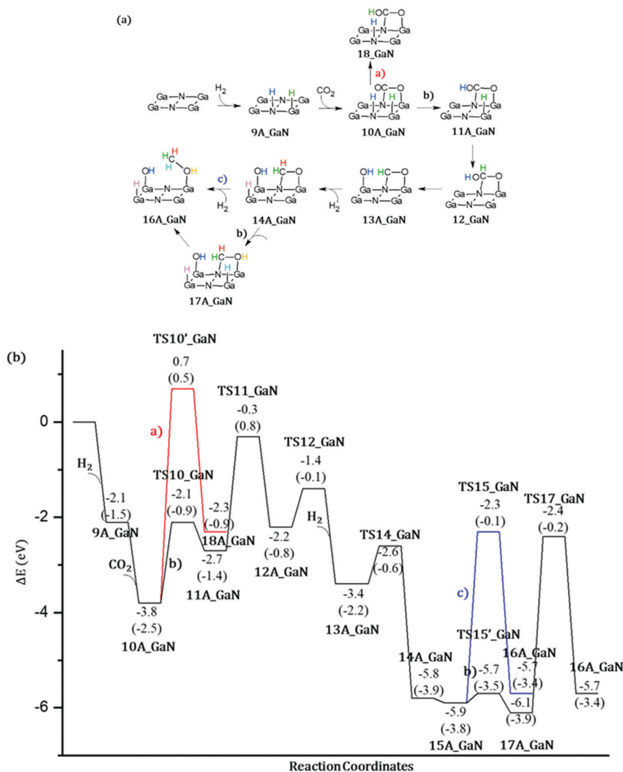
Fig. 6 (a) Schematic representations of all the intercepted stationary points along with the (b) calculated B3LYP energy profile for the \text{CO}_2 conversion to methanol on the \text{A}_n\text{GaN} cluster model according to mechanism 2. Energies are in eV and relative to the asymptote of the reactant. Free energies (eV) are shown in parentheses.
