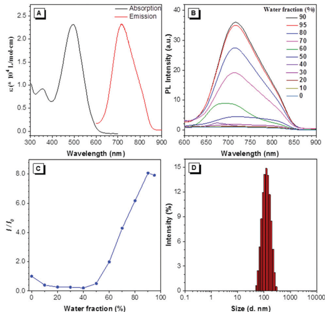
Fig. 1 General optical properties of DTZ-TPA-DCN . (A) Molar absorption and emission spectra of DTZ-TPA-DCN . (B) Photoluminescence (PL) intensity of DTZ-TPA-DCN (10 \mu\text{M} ) in mixtures of MeCN and water with different water contents. (C) Plots of the relative emission intensity of DTZ-TPA-DCN versus water fraction. I_0 and I are the peak values of the PL intensities of DTZ-TPA-DCN (10 \mu\text{M} ) in MeCN and MeCN/water mixtures, respectively. (D) Size distribution of DTZ-TPA-DCN in the mixture of MeCN/water with 90% water content.
