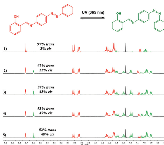
Fig. 4 1 H NMR spectrum (500 MHz, CDCl 3 ) of 1H showing spectral changes during UV irradiation: (1) prior to irradiation; (2) after 5 min; (3) after 10 min; (4) after 20 min and (5) after 30 min.
