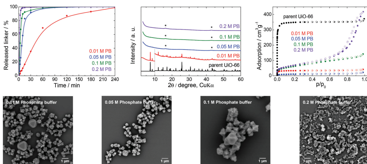
Fig. 4 The stability of UiO-66 in PB solutions at pH 7.5, a 4 h treatment. Upper row from left: Kinetics of the terephthalate release in PB of different concentrations, comparison of the PXR pattern of the parent UiO-66 with those of post-exposed specimens, and N_2 adsorption isotherms of the parent UiO-66 and of post-exposed specimens. The PXR patterns have been normalized and shifted vertically to avoid overlaps and the vertical dashed line divides the diffractograms at 2\theta = 10^\circ so that the less intensive diffractions above 10^\circ can be enlarged. The diffraction lines marked with an asterisk resulted from the Mylar foil support. Bottom row: SEM images of UiO-66 samples after immersion in PB solutions of varying concentrations (see Fig. 2 for an SEM image of the parent UiO-66).
