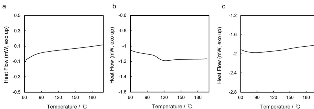
Fig. 4 DSC curves of (a) lin -poly(1,4Si 6 ), (b) cyc -poly(1,3Si 6 ), and (c) lin -poly(1,3Si 6 ). The second cycle is shown. Heating rate: 3 °C min -1 for lin -poly(1,4Si 6 ), 20 °C min -1 for cyc -poly(1,3Si 6 ) and lin -poly(1,3Si 6 ).
