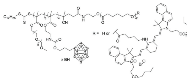
Fig. 4 Structure of the amphiphilic poly(carborane-containing methacrylate)- b -poly( \epsilon -caprolactone) with or without a near-infrared amino-cyanine dye.
