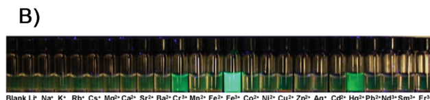
Fig. 4 (A) Cryptand-bodipy based sensor 7 for the detection of \text{Fe}^{3+} . (B) Naked-eye fluorescence responses of 7 ( 7\ \mu\text{M} ) in \text{H}_2\text{O}-\text{CH}_3\text{CN} (9:1) upon addition of 100 equiv. of various metal cations ( \lambda_{\text{ex}} = 365\ \text{nm} ). Reproduced with permission from ref. 29, copyright American Chemical Society.
