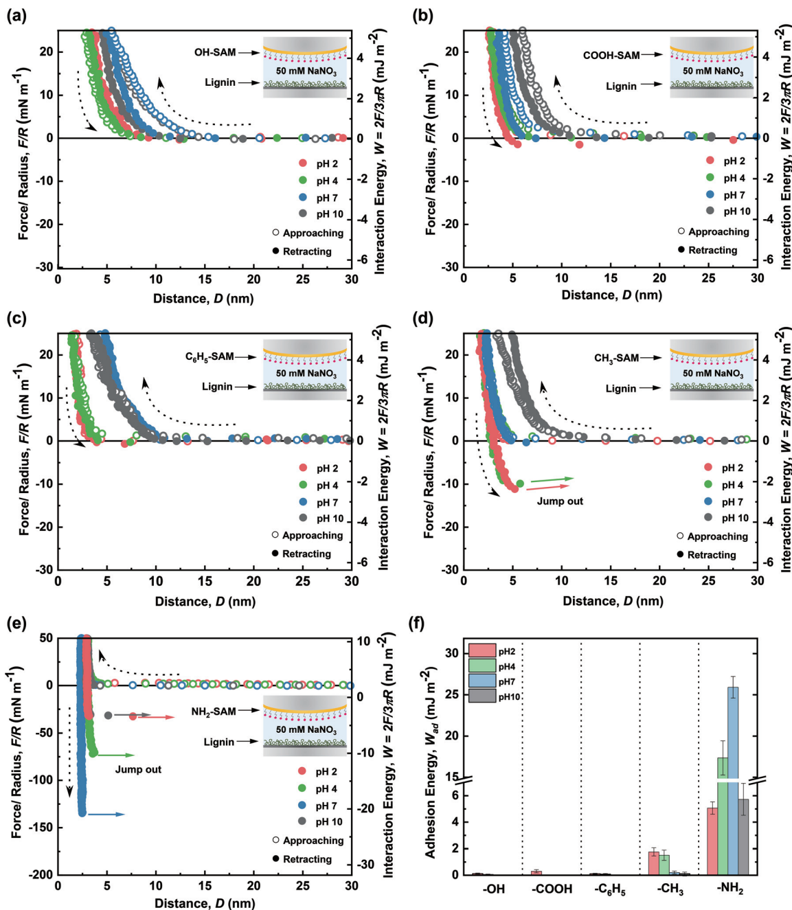
Fig. 2 Force–distance profiles between lignin nanofilms and SAMs terminated by various functional groups [(a) –OH, (b) –COOH, (c) – \text{C}_6\text{H}_5 , (d) – \text{CH}_3 , and (e) – \text{NH}_2 ] in pH 2, 4, 7, and 10 solutions. (f) Bar graph summarizing the overall adhesion energy ( W_{ad} ) for each curve.
