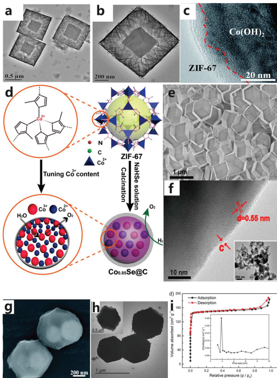
Fig. 3 (a and b) TEM images of \text{Co}(\text{OH})_2 -1. 64 Copyright © 2019 Elsevier Inc. All rights reserved. (c) HRTEM images of the EG/ \text{Co}(\text{OH})_2 /ZIF-67 hybrid. 65 Copyright © 2018, Royal Society of Chemistry. (d) Schematic diagram of the synthesis of \text{Co}_{0.85}\text{Se}@\text{C} nanoparticles. (e) SEM image of ZIF-67. (f) HRTEM image of ZIF- \text{Co}_{0.85}\text{Se} . Inset: low-resolution TEM image. 66 Copyright © 2016, American Chemical Society. (g) SEM images of ZIF-67@ \text{Fe}_3\text{O}_4 nanoparticles. 67 Copyright © 2019, Royal Society of Chemistry. (h) TEM images of HHTP@ZIF-67. (i) The Brunauer–Emmett–Teller (BET) specific surface area and the corresponding pore size distribution plot (inset) of HHTP@ZIF-67. 46 Copyright © 2018 Wiley-VCH Verlag GmbH & Co. KGaA, Weinheim.
