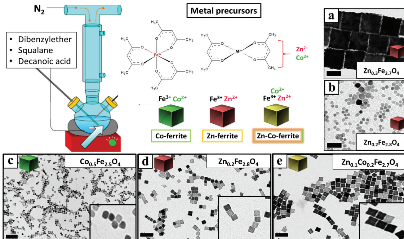
Fig. 2 BF-TEM images of mixed ferrite NCs: (a) Zn 0.3 Fe 2.7 O 4 NCs 65 \pm 5 nm; (b) Zn 0.2 Fe 2.8 O 4 NCs 9 \pm 3 nm; (c) Co 0.5 Fe 2.5 O 4 NCs 12 \pm 1 nm; (d) Zn 0.2 Fe 2.8 O 4 NCs 12 \pm 1 nm; (e) Zn 0.1 Co 0.2 Fe 2.7 O 4 NCs 15 \pm 1 nm. These NCs were prepared by using different feed ratios of Zn/Co metal precursors [Zn(acac) 2 and Co(acac) 2 ], (a–b–d) only Zn(acac) 2 , (c) only Co(acac) 2 , and (e) Zn(acac) 2 and Co(acac) 2 . In all synthesis the total amount of metal precursors was fixed at 1.5 mM with Fe(acac) 3 fixed at 1 mM. The DA surfactant was fixed at (a) 8 mmol or (b) 6 mmol or (c) 7 mmol. All the other reaction parameters were identical (100 mL flask, nitrogen flow at 40 b per min). Scale bars (in black) indicate 50 nm in all images.
