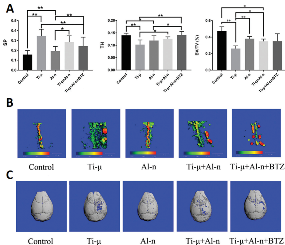
Fig. 7 Aseptic bone loosening induced by Ti-μ was prevented by Al-n particles, and BTZ was administrated in mouse model. A: The trabecular thickness and porosity percentage in a region of interest (ROI) of 1.5 \times 1.5 mm in the surgical area of the cranium harvested from C57BL/6 mice (groups: control, Ti-μ (10 mg of Ti-μ particles), Al-n (10 mg of Al-n particles), 10 mg of Ti-μ mixed with Al-n (Ti-μ:Al-n = 1:1), and 10 mg of Ti-μ mixed with Al-n administrated with 120 μL BTZ locally every two days (Ti-μ:Al-n = 1:1)) were measured and statistical analysed. (* P < 0.05 and ** P < 0.01 ). B: 3D reconstruction of the porosity images of the ROI of 1.5 \times 1.5 mm in each group. C: 3D reconstruction of the mouse calvaria in each group. (SP: trabecular spacing, TH: trabecular thickness, BV/TV: bone volume/total volume).
