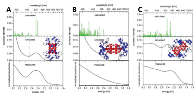
Fig. 16 A comparison of measured electronic spectra (powdered crystals in mineral oil) of (A) [Cu 12 S 6 (PPh 2 Et) 8 ], (B) [Cu 20 S 10 (PPh 3 ) 8 ] and (C) [Cu 24 S 12 (PEt 2 Ph) 12 ] with calculated singlet excitation energies and oscillator strengths plotted as vertical green lines as well as by superimposed Gaussians of fwhm = 0.3 eV (black) to simulate the experimental spectrum. The contributions of occupied orbitals are plotted in red, and those of the unoccupied orbitals are in blue. Reprinted with permission from ref. 165. Copyright 2015 American Chemical Society.
