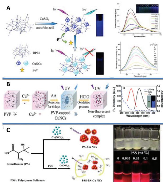
Fig. 2 (A) Synthesis strategy for the BPEI-CuNCs, their stability under varying pH and the mechanism of the branched polyethylenimine (BPEI)-CuNCs probe for Fe 3+ sensing. Reprinted with permission from ref. 30. Copyright 2015 Elsevier. (B) Schematic diagram of PVP-capped CuNCs (on the left) and UV-vis absorption, emission, and excitation fluorescence spectra of the probe CuNCs at pH = 6.2 in 50 mM phosphate buffer (PB) (on the right). Inset: Photograph of CuNCs probe in buffer under daylight (left) and UV-light (λ = 365 nm, right), respectively. Reprinted with permission from ref. 34. Copyright 2020 American Chemical Society. (C) A scheme depicting a plausible mechanism for the synthesis of PSS-stabilized penicillamine (PA)-CuNCs and the photographs of the PSS-PA-CuNCs synthesized under different concentrations of PSS, from 0.005 to 0.5 wt%. Adapted with permission from ref. 35. Copyright 2016 Springer Nature.
