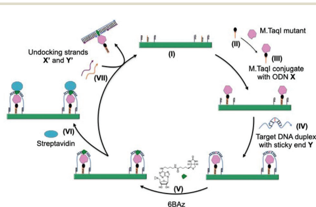
Fig. 1 Schematic flow of the machine cycle for the enzyme nano-factory and product detection after the addition of streptavidin.
