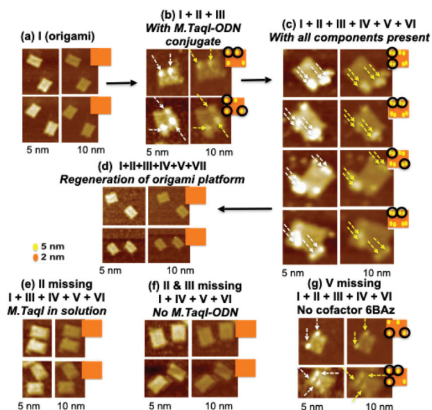
Fig. 2 AFM images of stepwise operation of a complete enzyme nano-factory cycle: (a) origami platform (I) only; (b) upon addition of the M-TaqI-ODN conjugate (II + III); (c) upon addition of the M-TaqI-ODN conjugate (II + III), target DNA (IV), 6BAz cofactor (V) and streptavidin (VI); (d) upon addition of the M-TaqI-ODN conjugate (II + III), target DNA (IV), 6BAz cofactor (V), undocking strands X' and Y' (VII). Control experiments: (e) M-TaqI is not embedded on the origami surface but free in solution; (f) M-TaqI and conjugated DNA both are missing; (g) cofactor 6BAz is missing. Schematic drawings next to AFM images show the expected height profile in (a)–(g). Schematic height profiles are shown with color coding, orange 2 nm; yellow 5 nm height and spots observed on individual origami are encircled.
