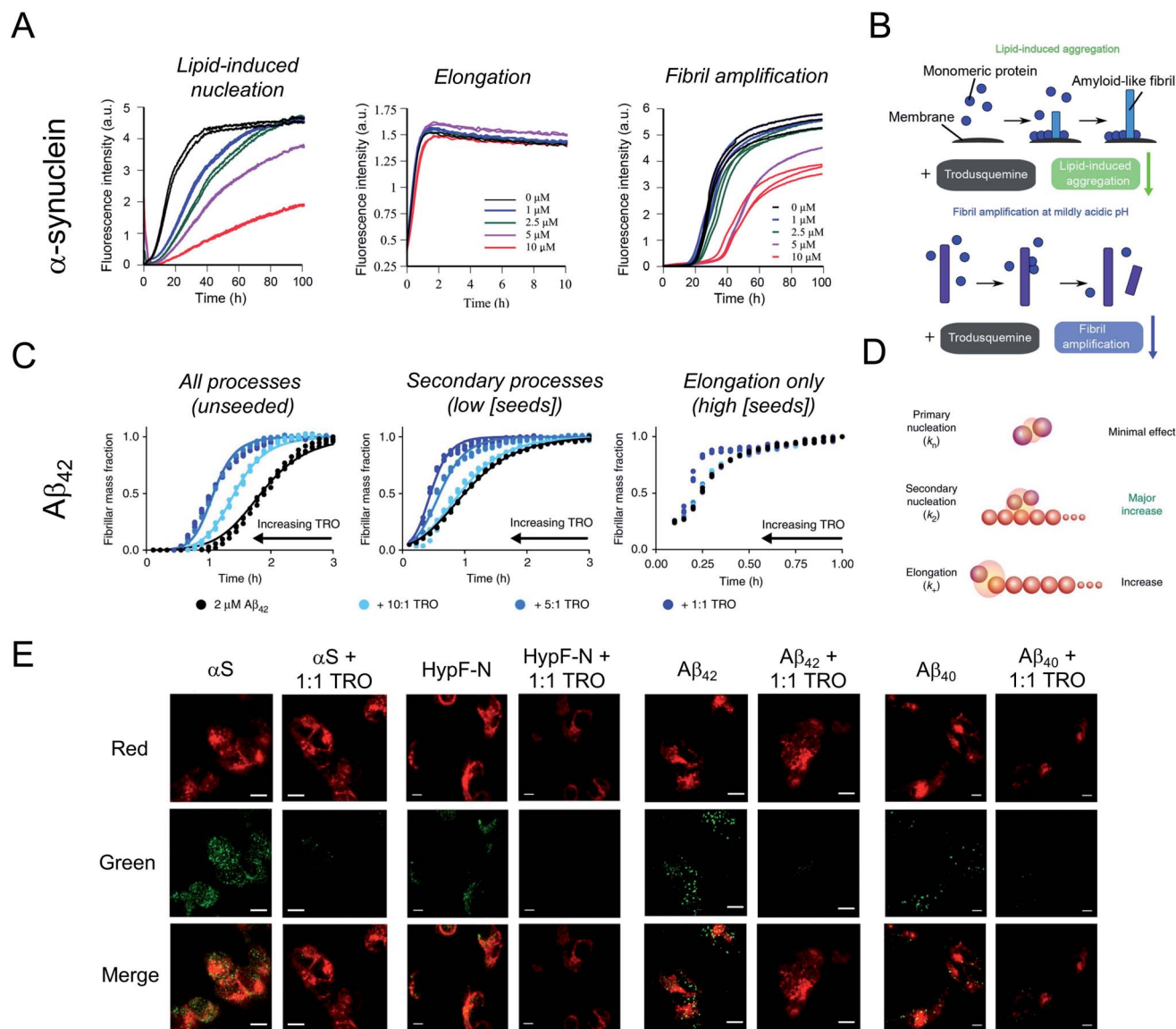
Fig. 2 Impact of trodusquemine on \alpha -synuclein and A \beta_{42} aggregation. (A) Trodusquemine (TRO) inhibits the lipid-induced nucleation and fibril amplification reactions in \alpha -synuclein aggregation, corresponding to primary and secondary nucleation events, respectively, without impacting fibril elongation. (B) Schematic representation of the effect of trodusquemine on the microscopic steps governing \alpha -synuclein aggregation under these conditions. (C) Trodusquemine accelerates the unseeded and seeded aggregation reactions of A \beta_{42} to varying degrees. (D) Schematic representation of the effect of trodusquemine on the microscopic steps governing A \beta_{42} aggregation under these conditions. (E) Confocal microscopy analysis of the extent of \alpha -synuclein, HypF-N, A \beta_{42} , or Zn 2+ -stabilized A \beta_{40} oligomer binding to the membranes of human neuroblastoma cells in the absence (left panels) or presence (right panels) of an equimolar concentration of trodusquemine shows that aminosterols induce the displacement of oligomers from cell membranes. Red and green channels indicate cell membranes and oligomers, respectively. Scale bars, 10 \mu m. Panels (A) and (B) and part of panel (E) were adapted with permission from M. Parni, P. Flagmeier, R. Limbocker, R. Cascella, F. A. Aprile, C. Galvagnion, G. T. Heller, G. Meisl, S. W. Chen, J. R. Kumita, P. K. Challa, J. B. Kirkegaard, S. I. A. Cohen, B. Mannini, D. Barbut, E. A. A. Nollen, C. Cecchi, N. Cremades, T. P. J. Knowles, F. Chiti, M. Zaslhoff, M. Vendruscolo and C. M. Dobson, ACS Chem. Biol. , 2018, 13 , 2308–2319. Copyright 2018 American Chemical Society. Panels (C) and (D) and part of panel (E) were adapted from R. Limbocker, S. Chia, F. S. Ruggeri, M. Parni, R. Cascella, G. T. Heller, G. Meisl, B. Mannini, J. Habchi, T. C. T. Michaels, P. K. Challa, M. Ahn, S. T. Casford, N. Fernando, C. K. Xu, N. D. Kloss, S. I. A. Cohen, J. R. Kumita, C. Cecchi, M. Zaslhoff, S. Linse, T. P. J. Knowles, F. Chiti, M. Vendruscolo and C. M. Dobson, Nat. Commun. , 2019, 10 , 225 published by Springer Nature. Part of panel (E) was adapted from R. Limbocker, B. Mannini, F. S. Ruggeri, R. Cascella, C. K. Xu, M. Parni, S. Chia, S. W. Chen, J. Habchi, A. Bigi, R. P. Kreiser, A. K. Wright, J. A. Albright, T. Kartanas, J. R. Kumita, N. Cremades, M. Zaslhoff, C. Cecchi, T. P. J. Knowles, F. Chiti, M. Vendruscolo and C. M. Dobson, Commun. Biol. , 2020, 3 , 1–10 published by Springer Nature.
