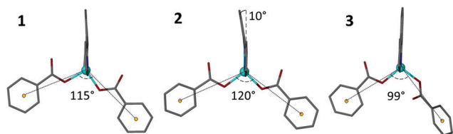
Fig. 4 A demonstration of hinge-like flexibility observed at the zinc coordination sphere for structures 1–3 . Both the angle, orientation and coordination mode of the H c bt ligand influences the size of the resulting channels within the motif. Angles are rounded to the nearest integer.
