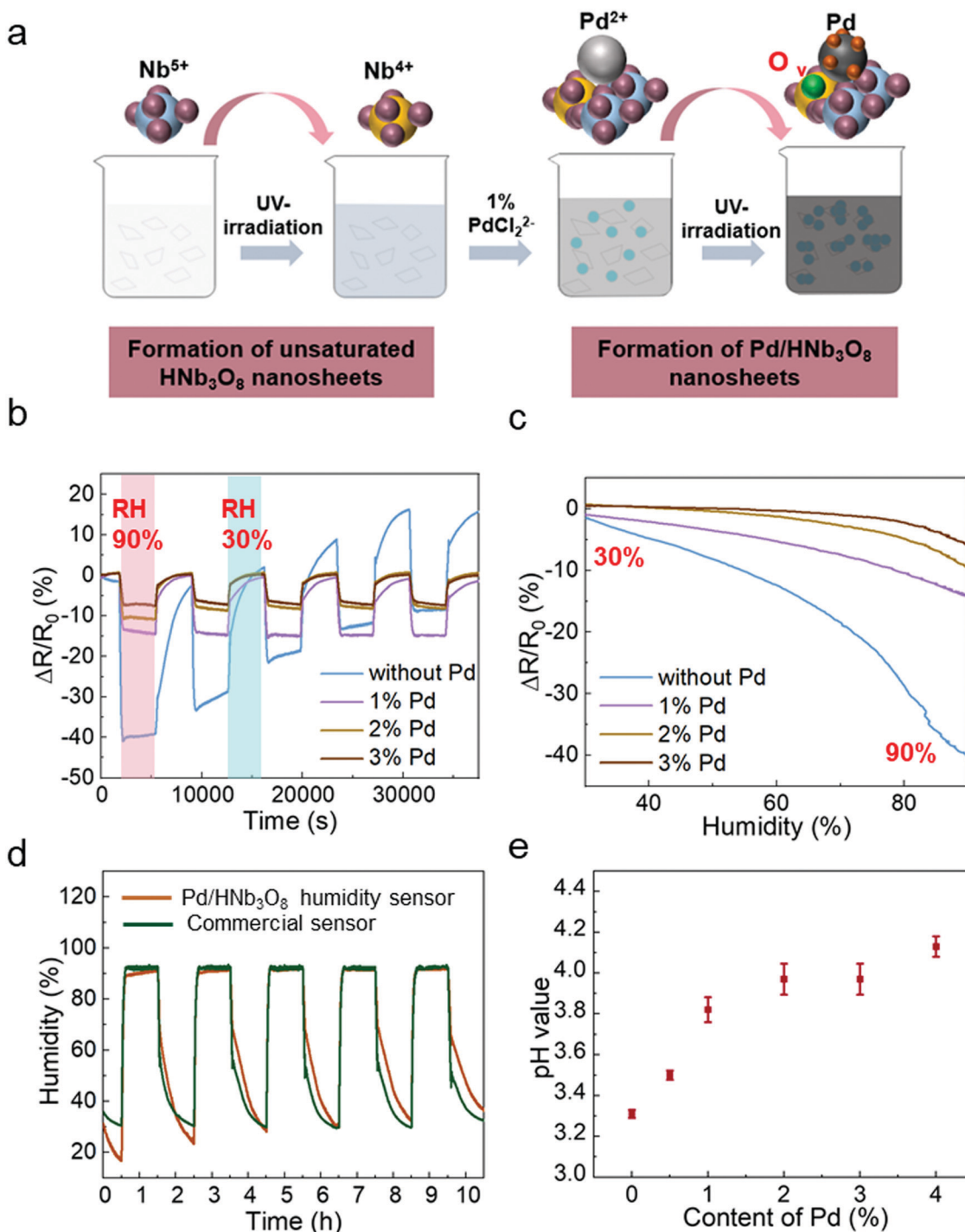
Fig. 2 (a) Overview of the synthesis of 1% Pd/ \text{HNb}_3\text{O}_8 nanosheets. (b) Cycling tests of \text{HNb}_3\text{O}_8 humidity sensors with different Pd contents and humidity variations from 30% to 90%. (c) Resistance change of different Pd contents of the Pd/ \text{HNb}_3\text{O}_8 humidity sensor as a function of RH. (d) Long-term cycling tests of a 1% Pd/ \text{HNb}_3\text{O}_8 humidity sensor compared with that of a commercial humidity sensor under the same RH. (e) pH results of the prepared \text{HNb}_3\text{O}_8 nanosheet solution with different Pd contents.
