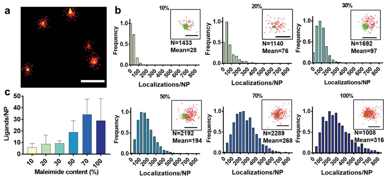
Fig. 2 (a) Representative DNA-PAINT image of ligand-conjugated PLGA-PEG (PEG 5k ) 50% maleimide NPs displaying the number of localizations (red) per NP (scale bar = 200 nm). The yellow signal is DiI dye encapsulated in NP, used for mechanical drift correction and as a reference in NP identification. (b) Normalized frequency histograms of DNA-PAINT localizations for PLGA-PEG-maleimide (long PEG 5k ) NP at various maleimide contents (10–100%), the number of NP analysed ( N ) and the mean number of localizations. Close-up images of representative NP for each formulation (scale bar = 100 nm), whereby DNA-PAINT localizations are seen in red and DiI in green. (c) The number of available ligands/NP per formulation as retrieved by qPAINT. The data were analysed using Matlab software.
