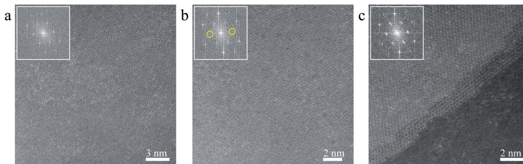
Fig. 2 ADF-STEM of a hollow WS 2 pyramid atomic resolution. Annular dark-field scanning transmission electron microscopy images taken in (a and b) the middle region, and (c). The side of a hollow WS 2 pyramid. Subtle variations in the atomic arrangement can be observed. The corresponding FFTs, as given as insets in each of the panels, highlight this feature further. Changes in the Bragg reflections occur between them. One of which is a reduction of the intensity of one of the Bragg reflections in the middle region of the hollow pyramid, as marked by the yellow circles in (b).
