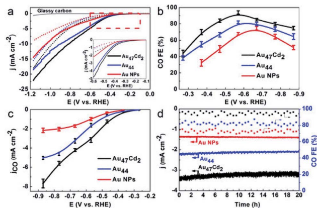
Fig. 12 (a) LSV curves of \text{Au}_{47}\text{Cd}_2(\text{TBTT})_{31} , \text{Au}_{44}(\text{TBTT})_{28} and the ca.1.5 nm Au NPs in an Ar-saturated (dotted line) and a \text{CO}_2 -saturated (full line) 0.5 M \text{KHCO}_3 solution; inset: enlarged LSV curves from @0.1 V to @0.6 V. (b) CO faradaic efficiency for the catalysts examined with different applied potentials. (c) The corresponding CO partial current density. (d) The stability test conducted at @0.57 V for \text{Au}_{47}\text{Cd}_2(\text{TBTT})_{31} and \text{Au}_{44} and at @0.67 V for the Au NPs. Reproduced with permission. 106 Copyright 2019 Wiley-VCH.
